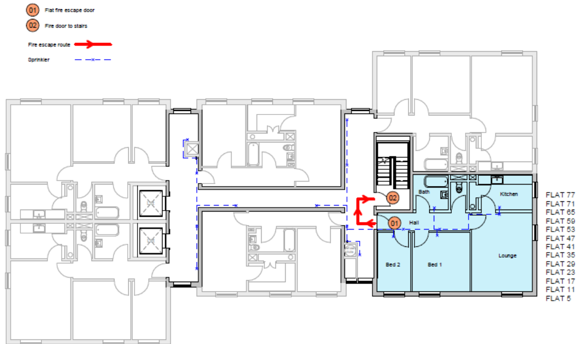
Fire Escape Layout Flat Type 4 1 : 100
