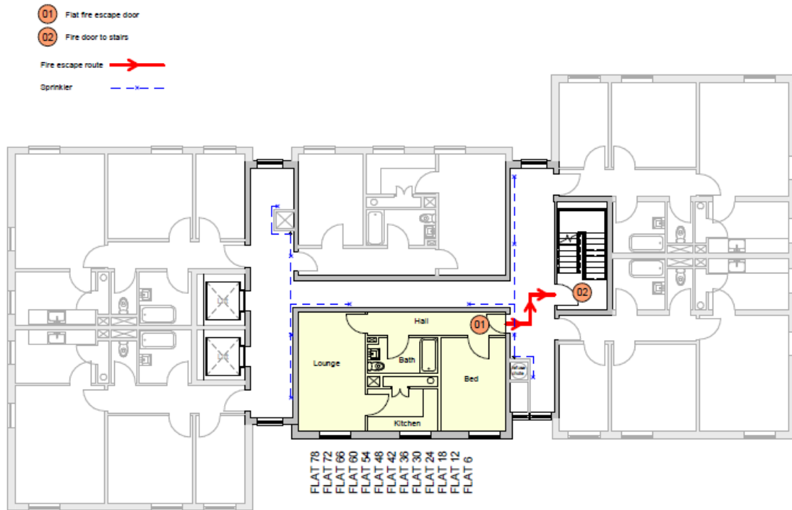
Fire Escape Layout Flat Type 5
