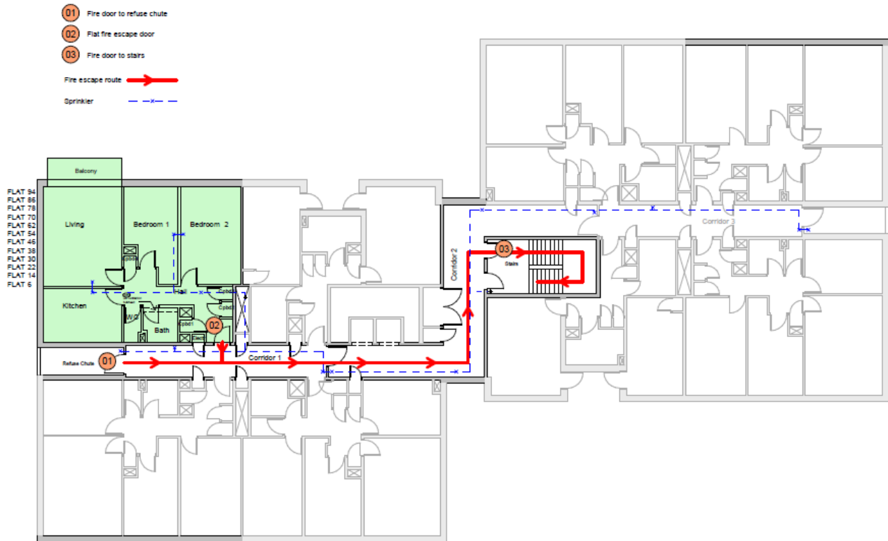
Fire Escape Layout Flat Type 1
