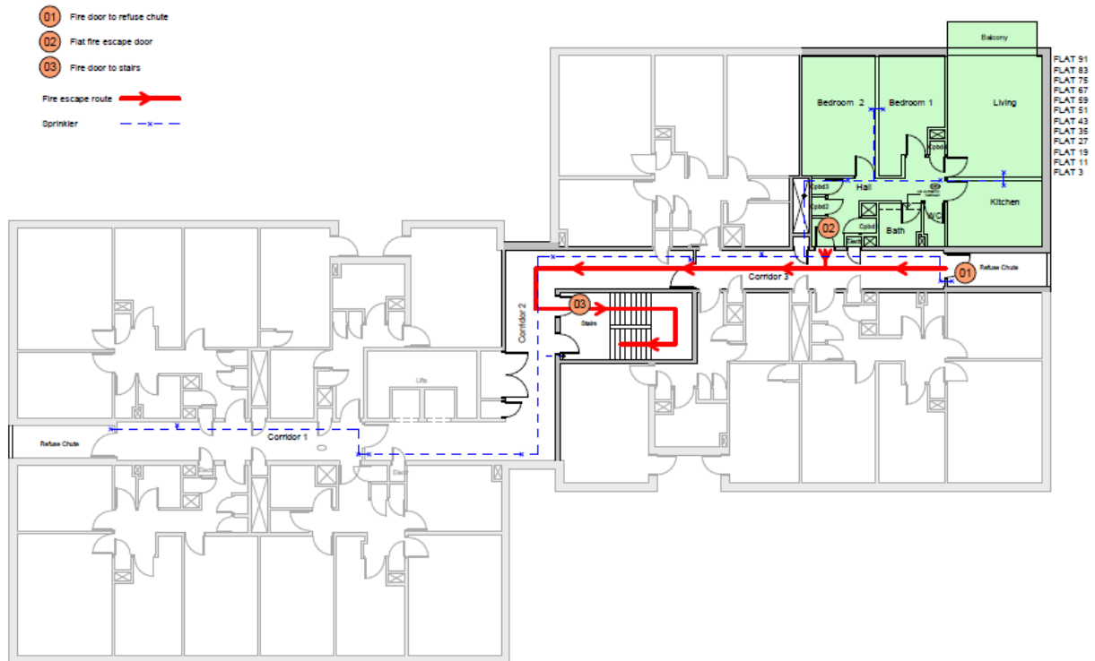
Fire Escape Layout Flat Type 4 1 : 100
