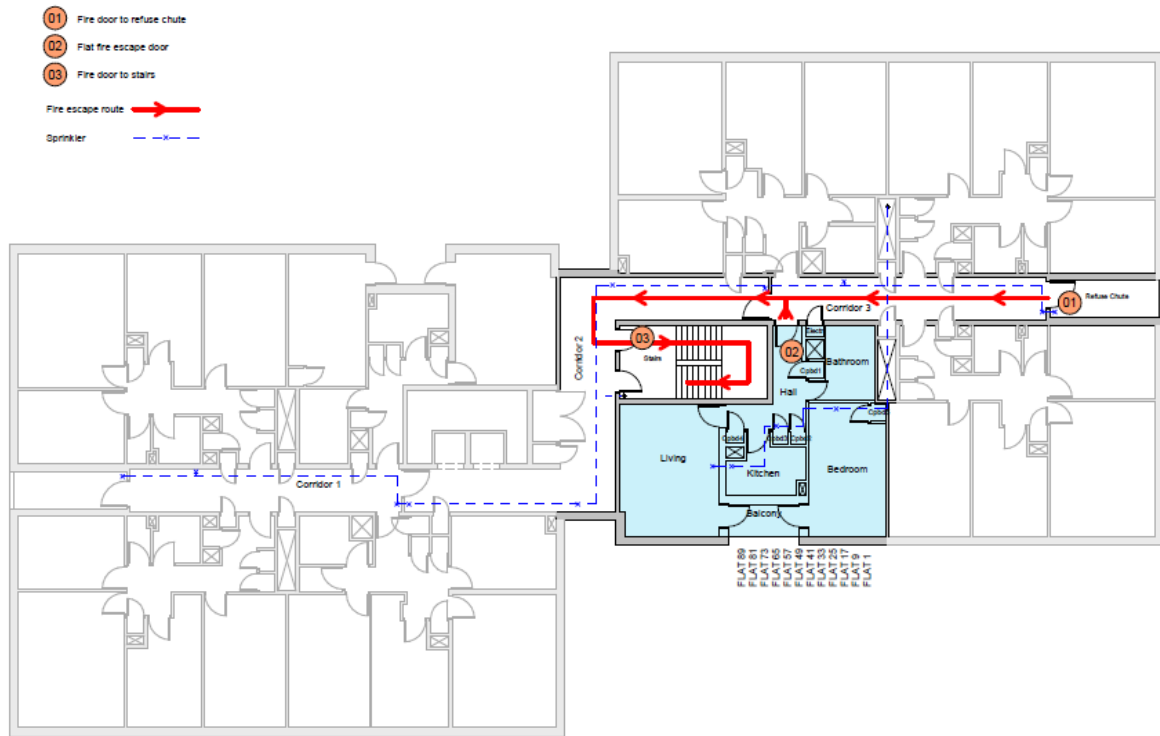
Fire Escape Layout Flat Type 6
