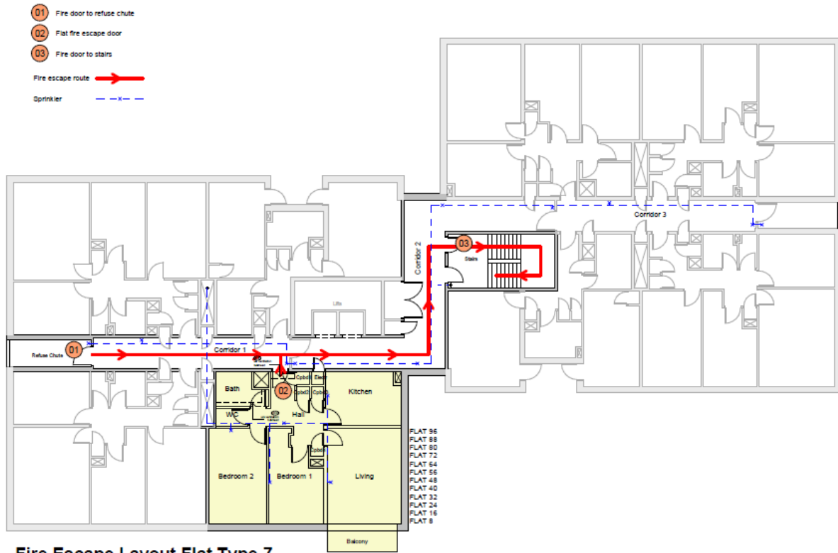
Fire Escape Layout Flat Type 7
