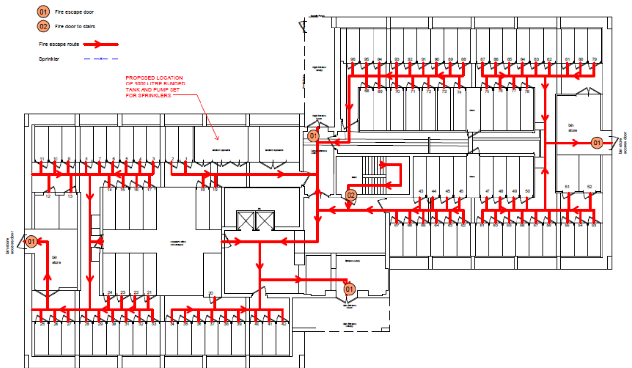
Ground Floor Fire Escape Layout 1:100
