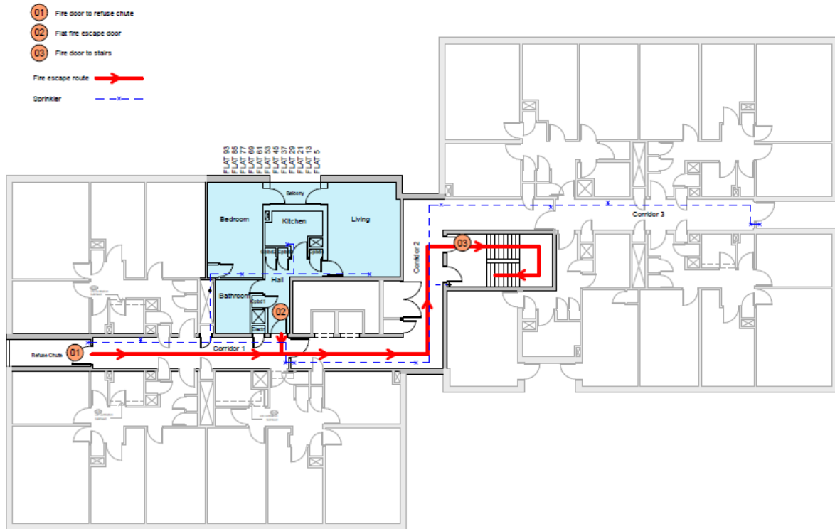
Fire Escape Layout Flat Type 2 1: 100
