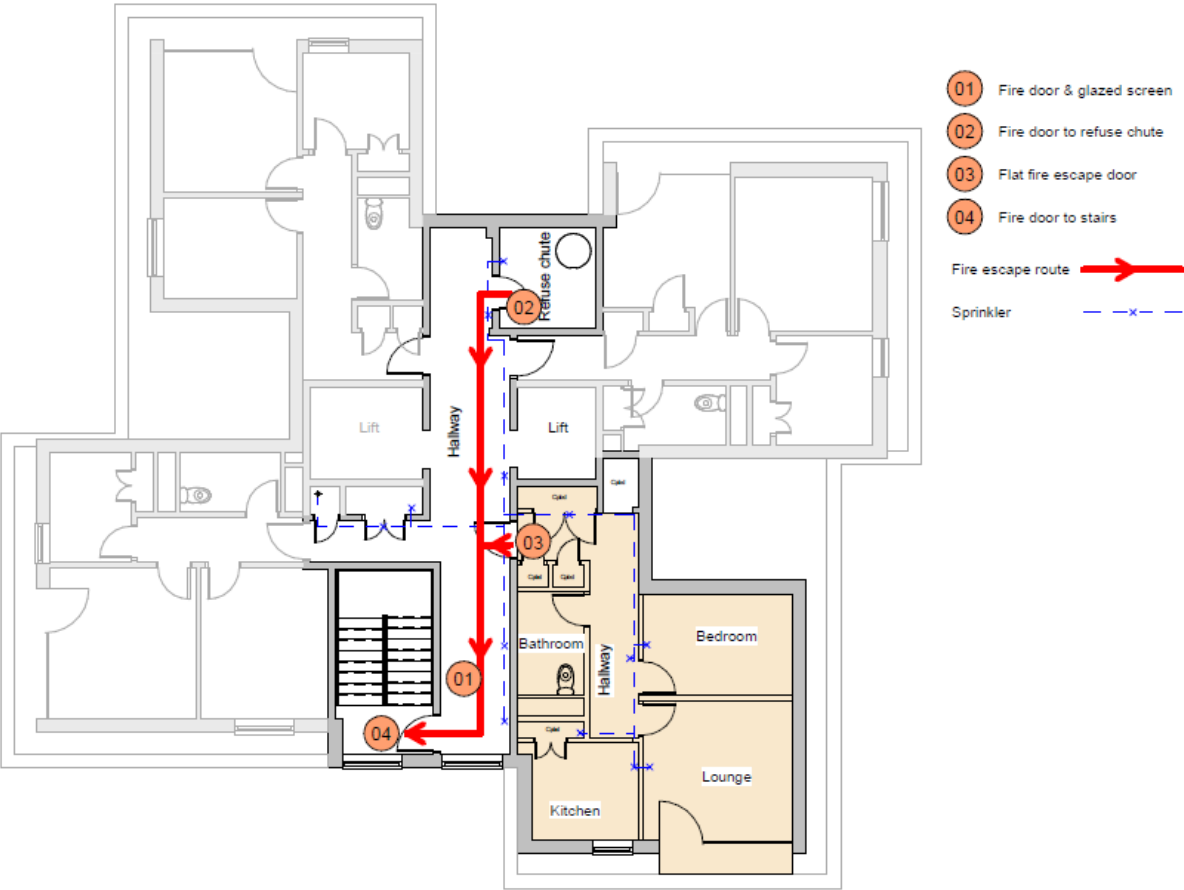
Fire Escape Layout Flat Type 7 1 : 100
