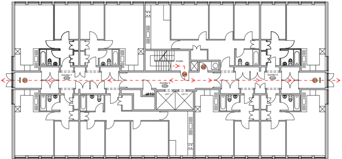
01 Fire Escape Route First Floor 1 : 100
