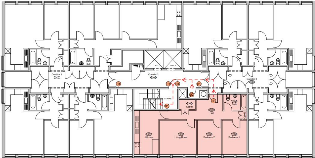
01 Fire Escape Layout Flat Type 6a 1 : 100
