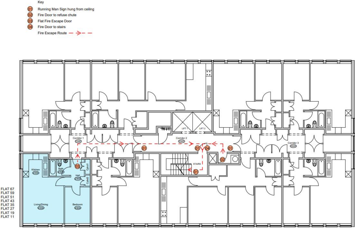
01 Fire Escape Layout Flat Type 8a 1 : 100
