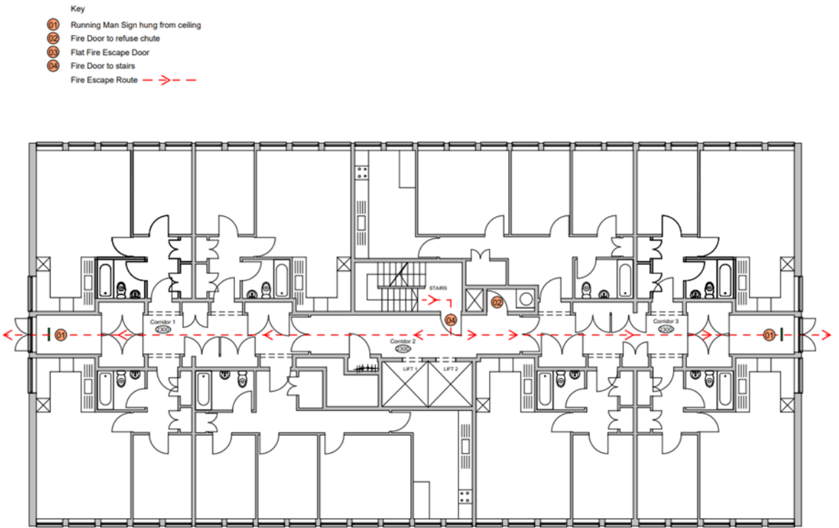
01 Fire Escape Route First Floor 1 : 100
