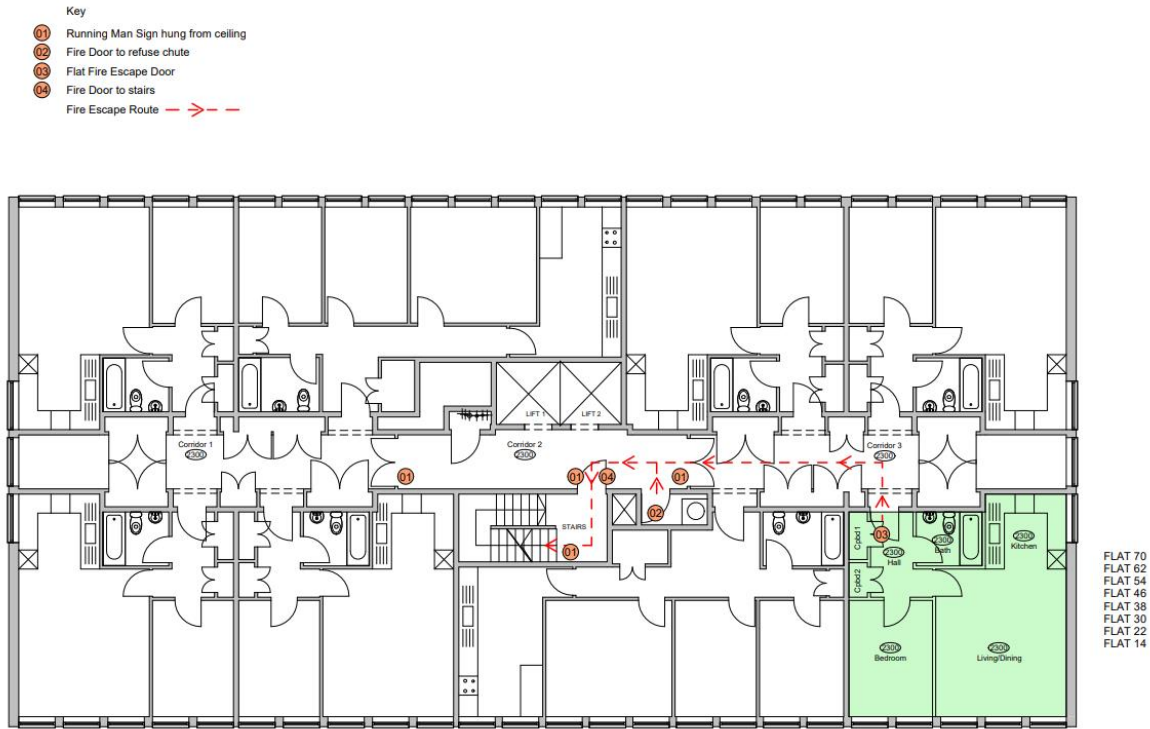
01 Fire Escape Layout Flat Type 5a 1 : 100
