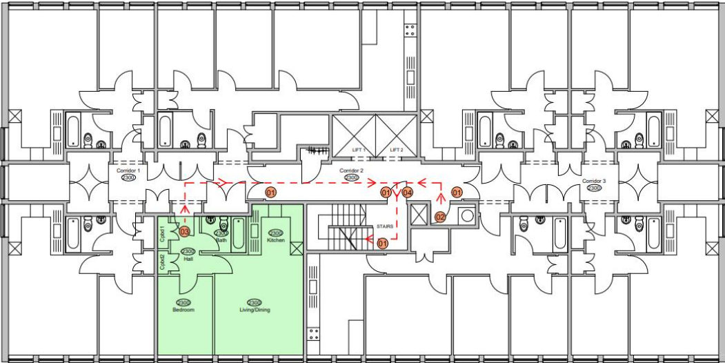
01 Fire Escape Layout Flat Type 7a 1:100
