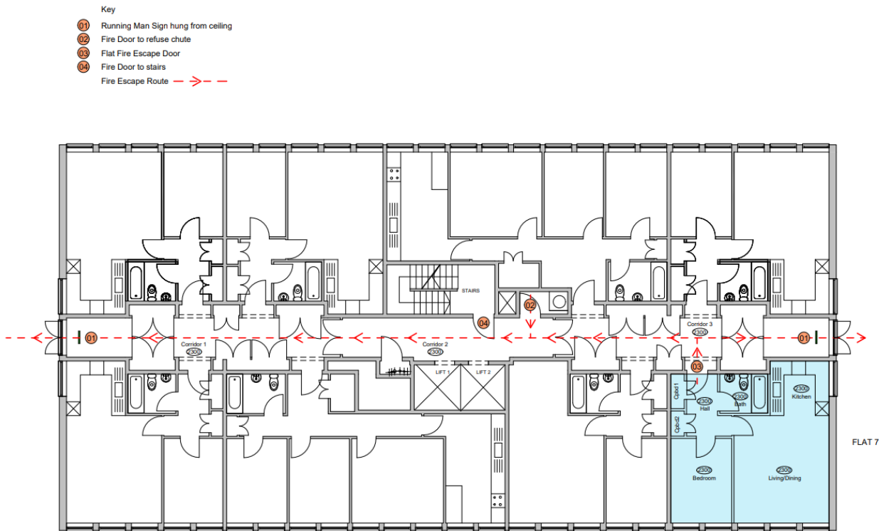
01 Fire Escape Layout FF Flat Type 5
