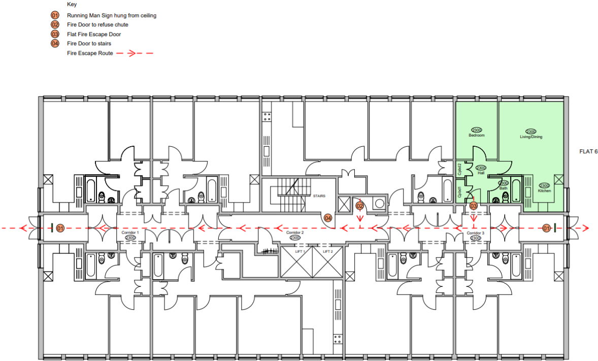
01 Fire Escape Layout FF Flat Type 4
