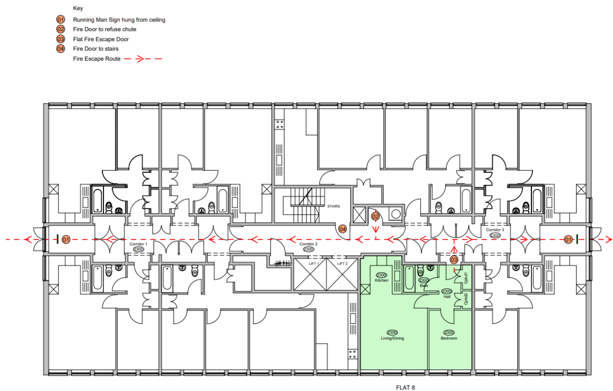
01 Fire Escape Layout FF Flat Type 6 1 : 100
