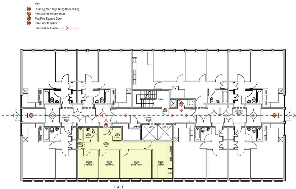
01 Fire Escape Layout FF Flat Type 7 1 : 100
