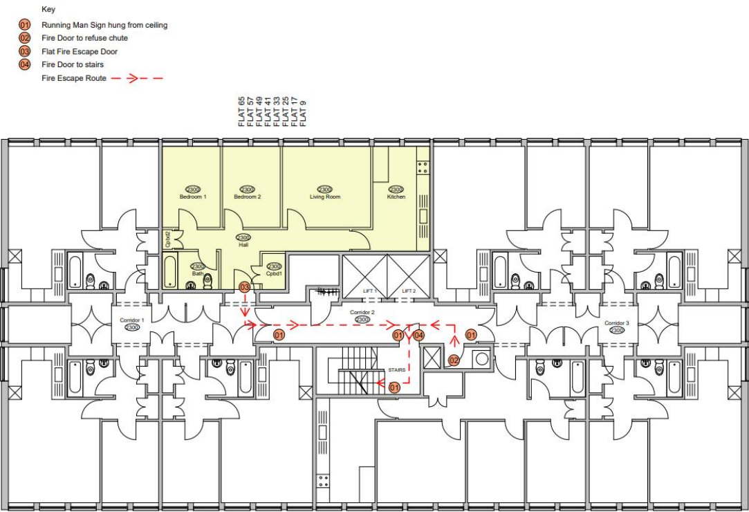
01 Fire Escape Layout Flat Type 2a 1 : 100
