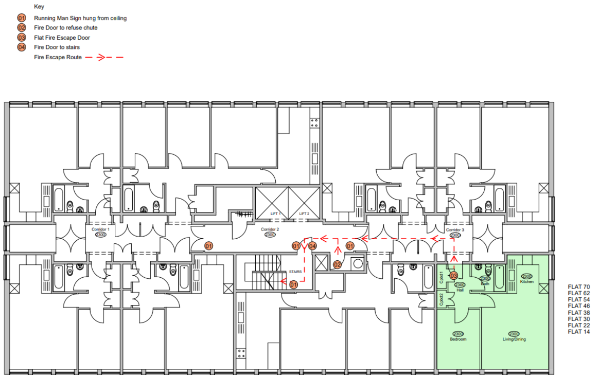
01 Fire Escape Layout Flat Type 5a
