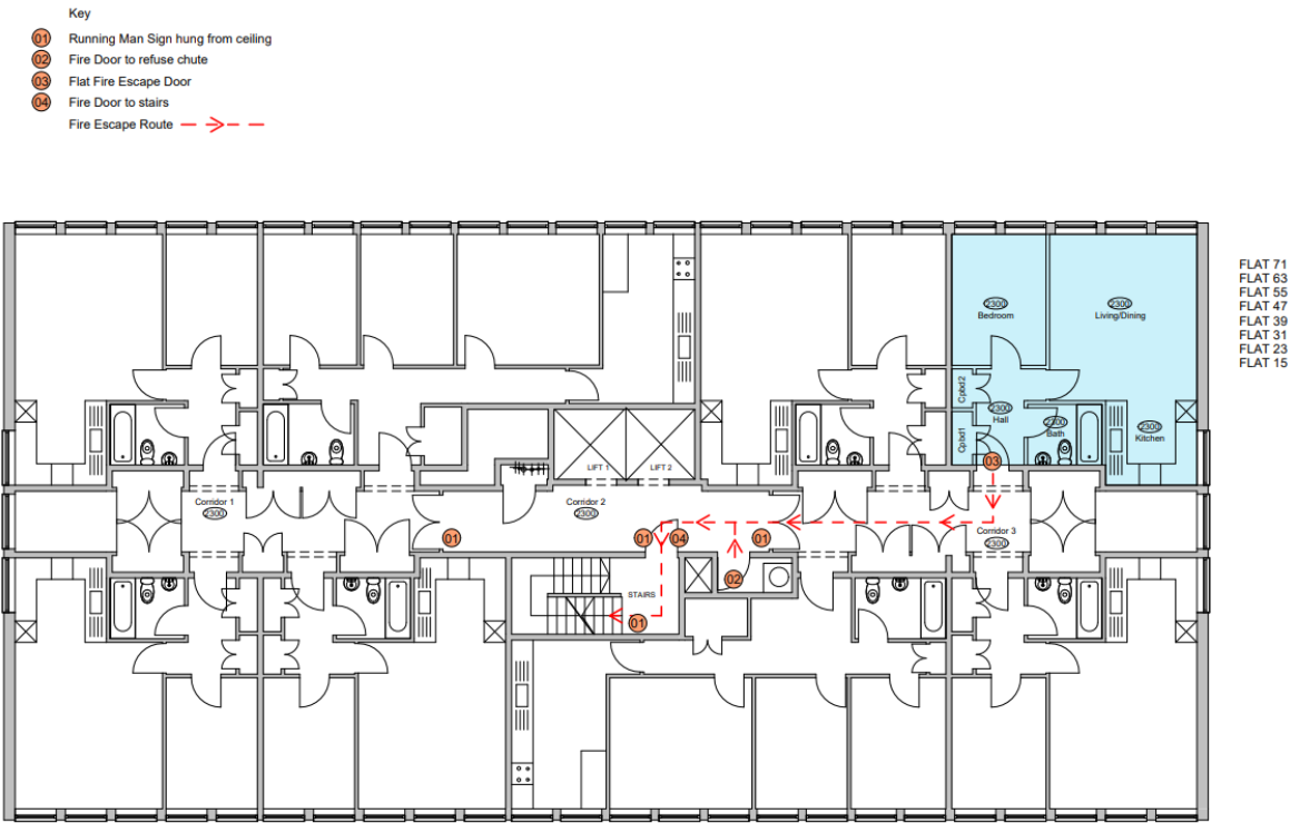
01 Fire Escape Layout Flat Type 4a 1 : 100
