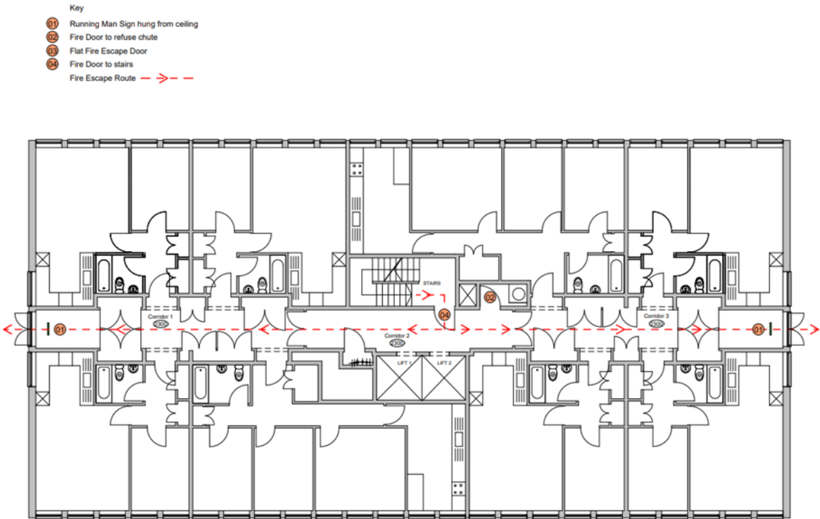
01 Fire Escape Route First Floor 1 : 100
