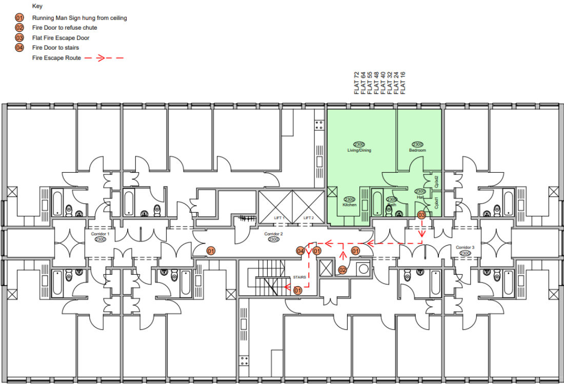
01 Fire Escape Layout Flat Type 3a 1 : 100
