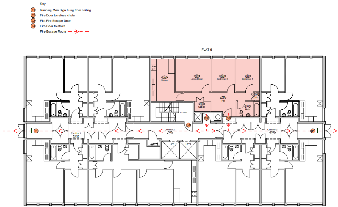
01 Fire Escape Layout FF Flat Type 3 1 : 100
