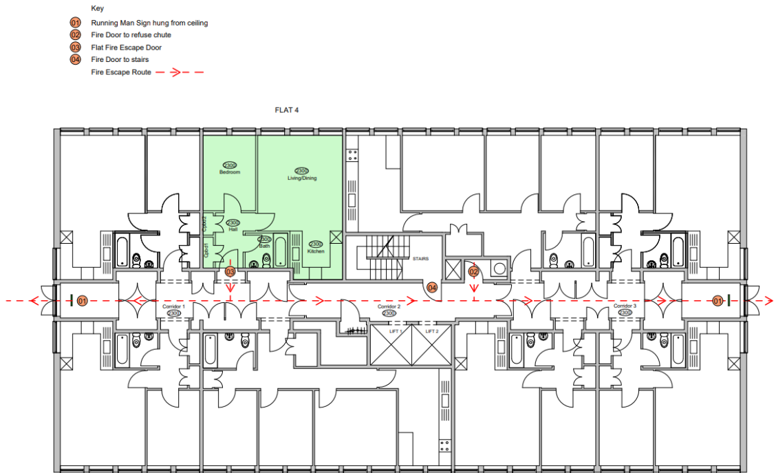
01 Fire Escape Layout FF Flat Type 2 1:100
