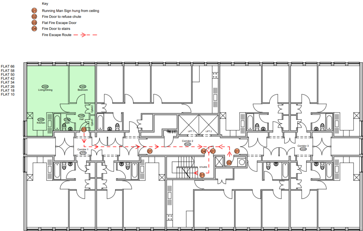
01 Fire Escape Layout Flat Type 1a
